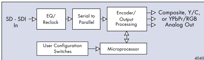
4040 Block Diagram
