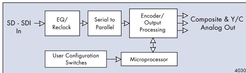
4030 Block Diagram
