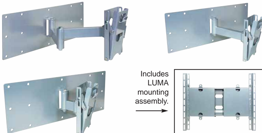
LUPM with LUMA • Holds 40" - 50" Plasma • 130 Lb. Capacity • 0°-10° Tilt • 42 Lbs.
