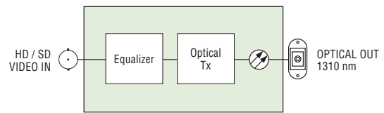
FEO-871p Functional Block Diagram
