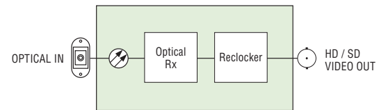
FOE-871p Functional Block Diagram
